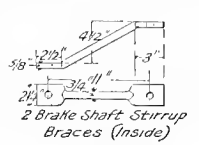
Figs. 1292-1293. Brake-shaft Stirrup Braces (2 of each).
